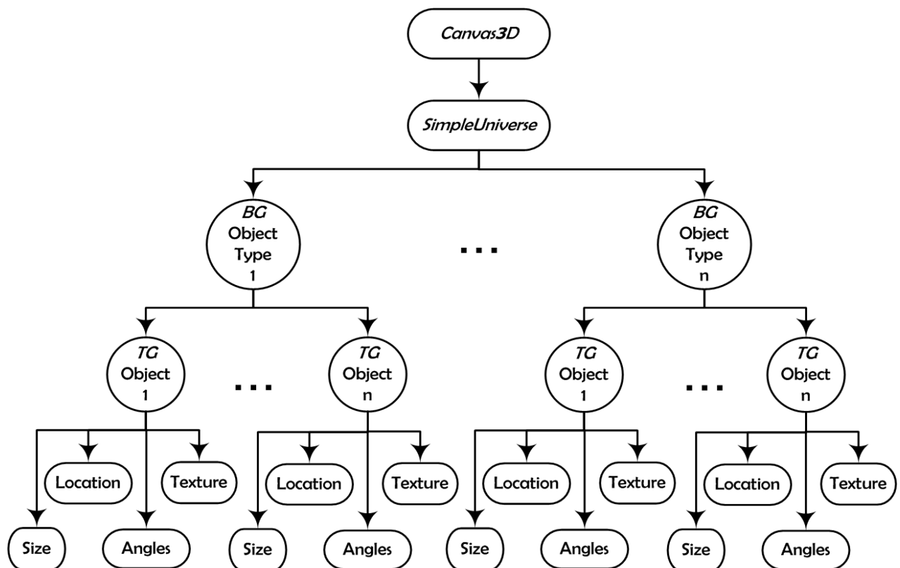
Fig. 4. 3D Model Generation in Java Environment
