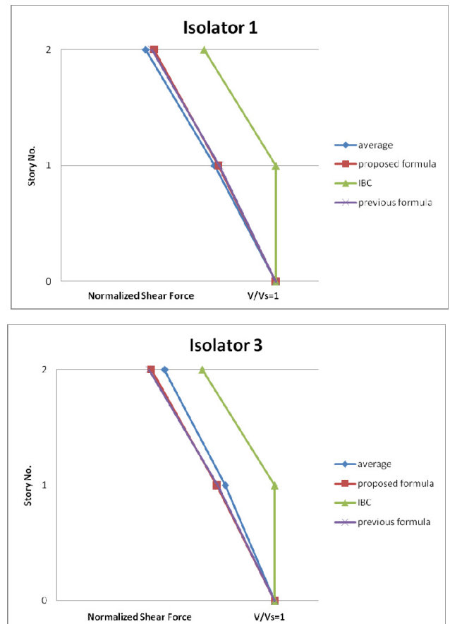
Fig. 9 Comparison of nonlinear dynamic analysis, IBC formula, proposed formula in section 6 and previous formula for 2 story building
