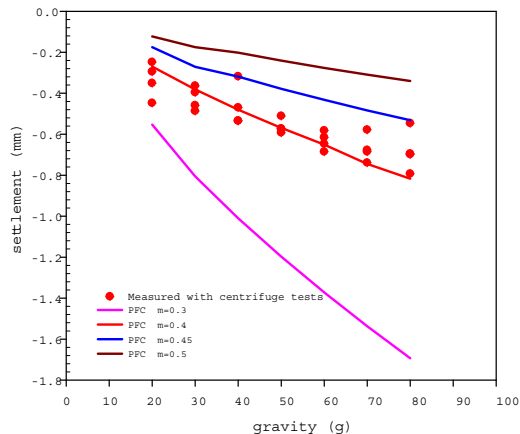
Fig. 16 Comparison of the calculated settlements of K_{no}=0.5 \times 10^7 N/m and various m ( m=0.3 , 0.4 , 0.45 , and 0.5 ) and the measured settlements from the physical modeling at various g-levels
