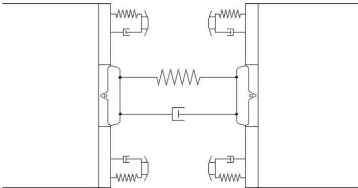
Fig. 2 Model of connection between wagons
